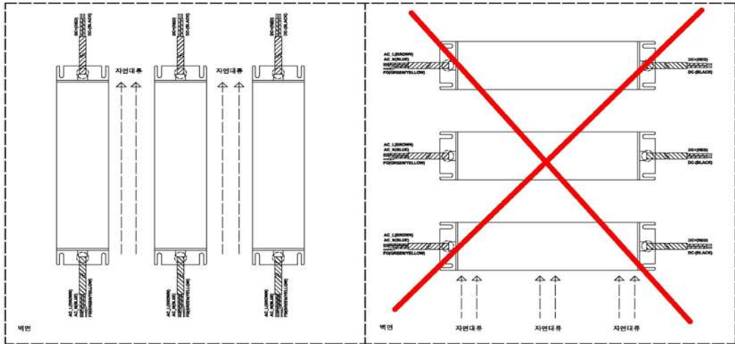
[Fig. 3] Installation method
