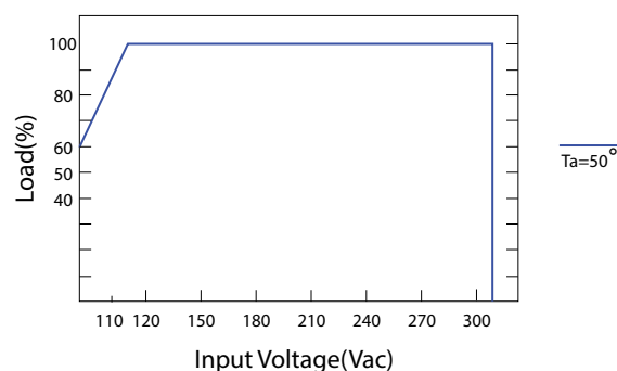
INPUT VOLTAGE VS LOAD
