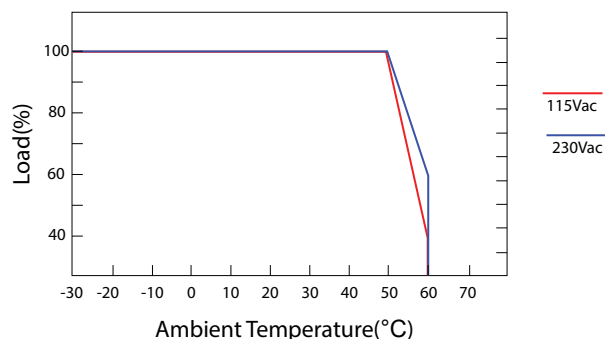
■ TEMPERATURE VS LOAD CURVE
